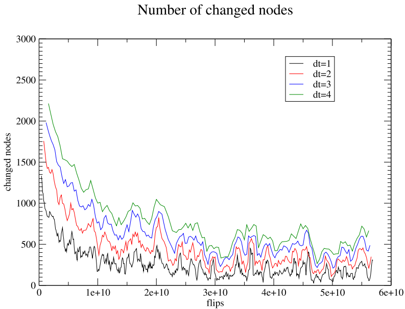
Fig. 14 (Color online) Number of nodes which differ between time t (in flips) and time t + 10^8 \cdot dt . The data are for n = 3283 and T = 0.175
