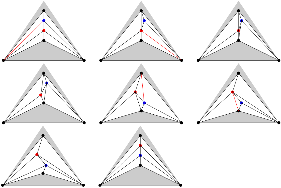
Fig. 4 (Color online) Exchanging blue and red in the stem of the Christmas tree by a sequence of moves. Top to bottom . The actual flips are taking place between frames 1–2, 2–3, 5–6, 6–7. The other transitions are again just moves for better visibility. Note that the shaded regions may contain arbitrary links, in particular, parts of the stem of the tree. Therefore, this sequence shows that any two positions in the vertical stem can be exchanged, except for the bottom 2. Those will be handled in Fig. 5
