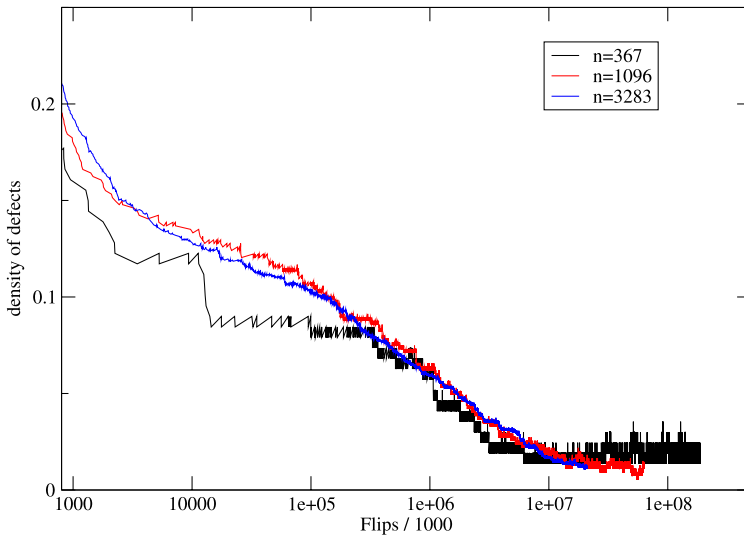
Fig. 12 (Color online) The energy as a function of the number of flips on approach to equilibrium (at temperature T = 0.175 ). The vertical scale is density of defects, i.e., defects/nodes. The horizontal axis is the number of flips, renormalized by 3283/n , i.e., the smaller triangulations converge faster than the larger ones. However, the slope is the same for the 3 cases. We have subtracted 6 from the energies, to take into account the 0 point energy (which is at least 6)
