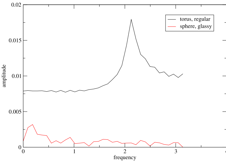
Fig. 16 (Color online) Power spectra for the torus triangulation and a glassy triangulation, corresponding to the equilibrium at T = 0.175
