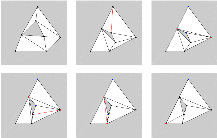
Fig. 9 (Color online) Motion of a defect by successive flips ( top row , then bottom row , left to right ). Shown is a sequence of moves which lowers the degree by 1 on the top node and raises the degree by one on the bottom left node, leaving in the end all other degrees intact. Flips take only place between frames 2–3, 4–5, and 5–6. The color code of the nodes is red for an increase of the degree by 1 and blue for decrease by one.
