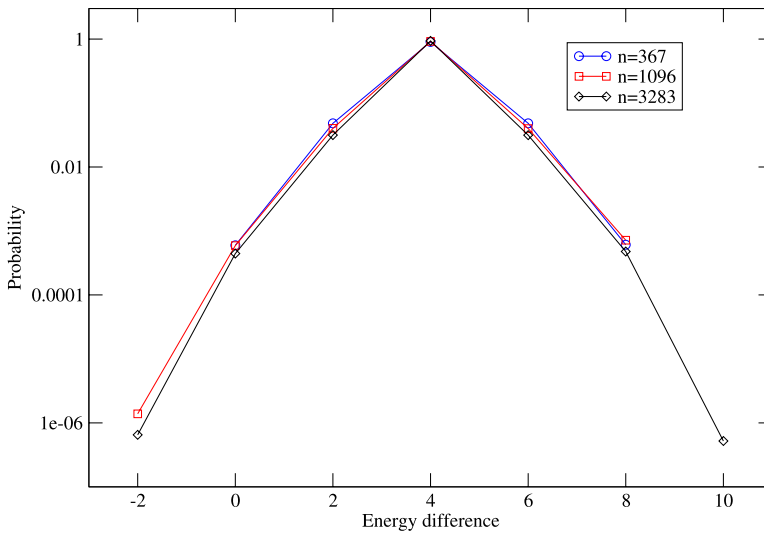
Fig. 13 (Color online) The neighborhood of typical glassy configurations. See the text for explanations
