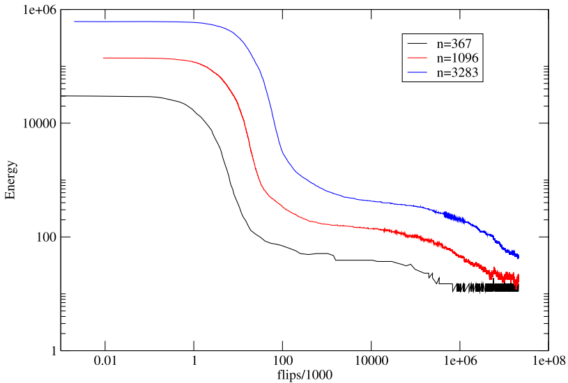
Fig. 10 (Color online) The energy as a function of the number of flips. The vertical scale is energy
