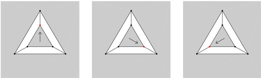
Fig. 8 (Color online) Three configurations, in the interior of an arbitrary triangle, which have the same energy (the inserted figure being one with three external nodes of same degree and same color). These three configurations are different unless the interior triangle has 3-fold symmetry
