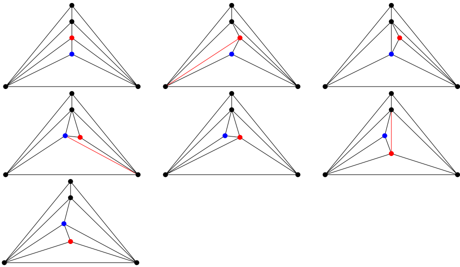
Fig. 5 (Color online) Exchanging blue and red in the two bottom positions of the Christmas stem. Top to bottom . The flips occur between frames 2–3, 4–5, and 6–7
