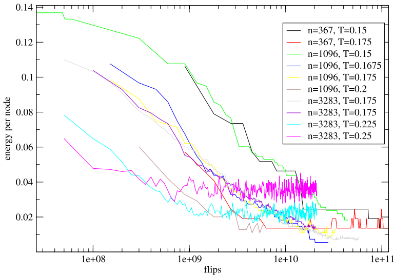
Fig. 11 (Color online) The data for n = 367, 1096, and 3283 and 1/\beta = T as shown in legend. The x-axis is the logarithm of number of attempted flips, normalized by 3283/n , and the y-axis energy per node after having subtracted a zero-point energy E_0 = 6 from all the energies. Note a certain data collapse for each temperature T , independent of size n
