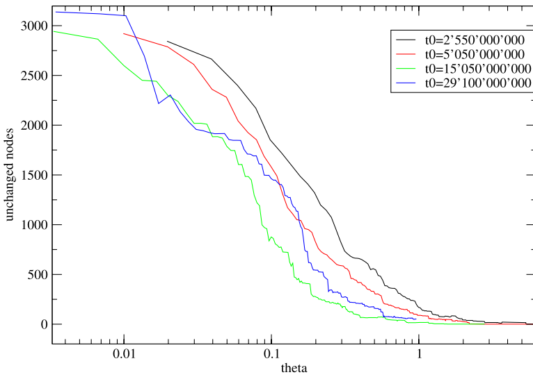
Fig. 15 (Color online) Number of nodes which are unchanged as a function of \theta = dt/t . The vertical axis is 3283 - D(t_0, t_0 + dt) , with t_0 given in the caption and D defined in the text. The data are for n = 3283 and T = 0.175 . Perfect data collapse would check the scaling relation f(\theta) = D(t_0, t_0 + \theta t_0)
